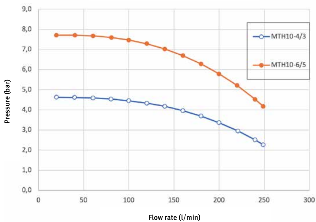
Pump Curve WT7-90
